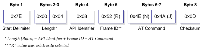
Figure 7-8. Example: API frames when modifying the NJ parameter value of the module.
