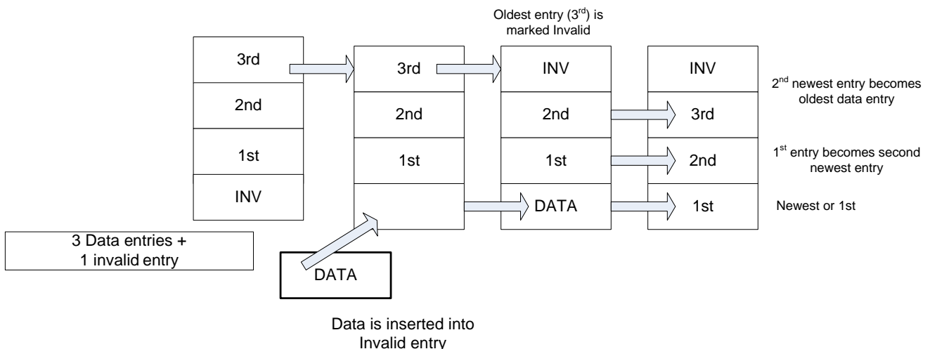
Figure 4-09. Demonstration of how entries in the received data bindings are replaced when an RF data packet is received.
