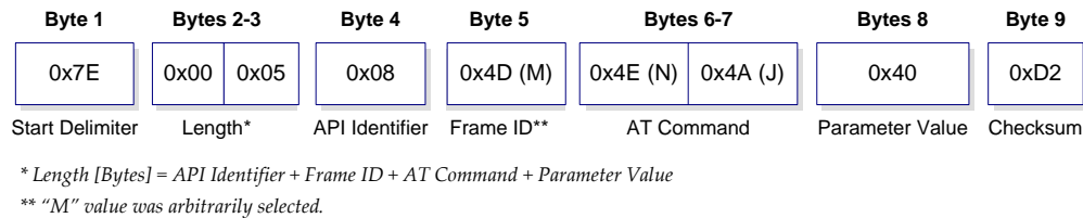
Figure 7-8. Example: API frames when modifying the NJ parameter value of the module.
