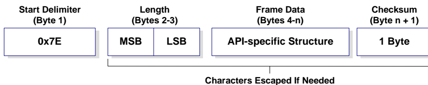
Figure 7-02. UART Data Frame Structure - with escape control characters:
