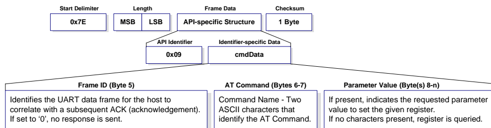
Figure 7-9. AT Command Frames (Note that frames are identical to the "AT Command" API type except for the API identifier.)
