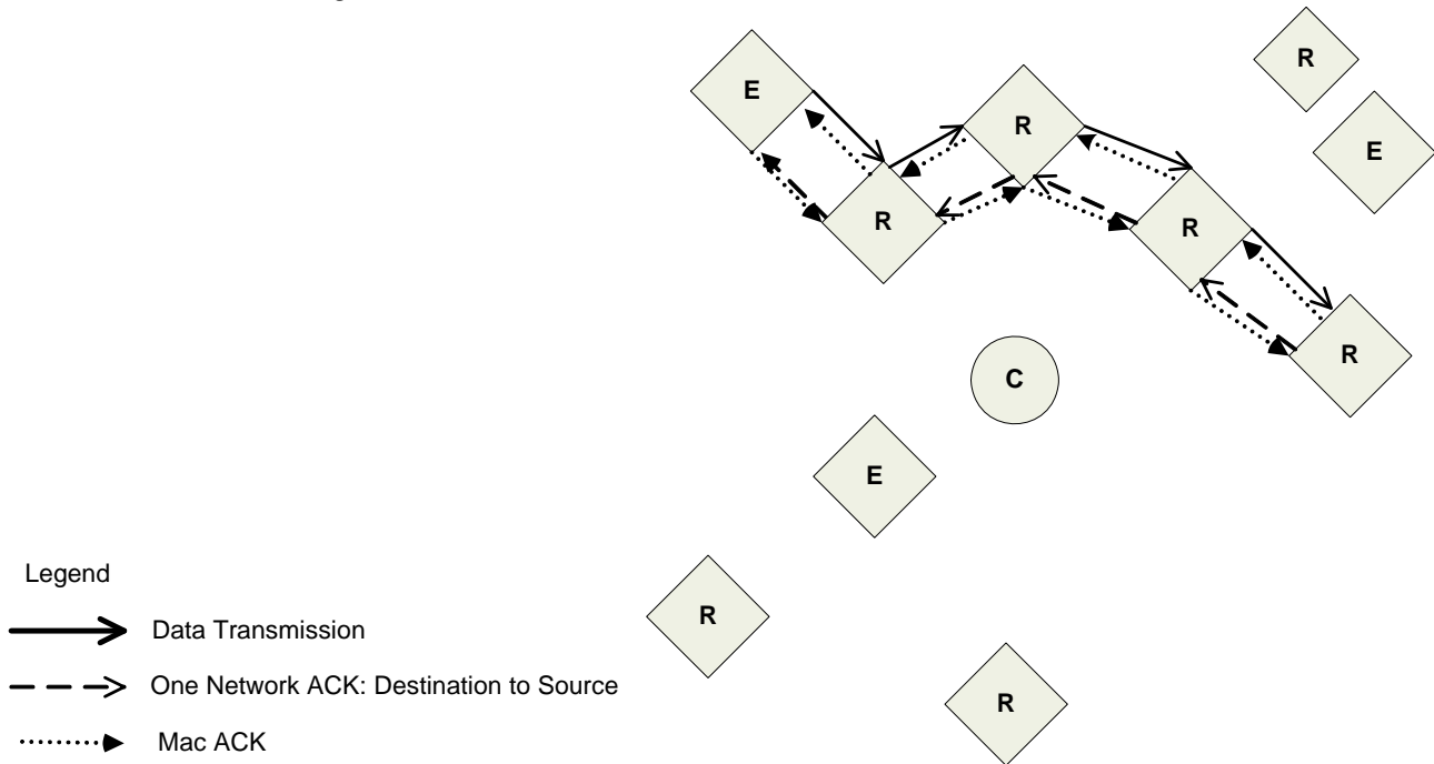
Figure 3-08. Unicast Data Transmission
